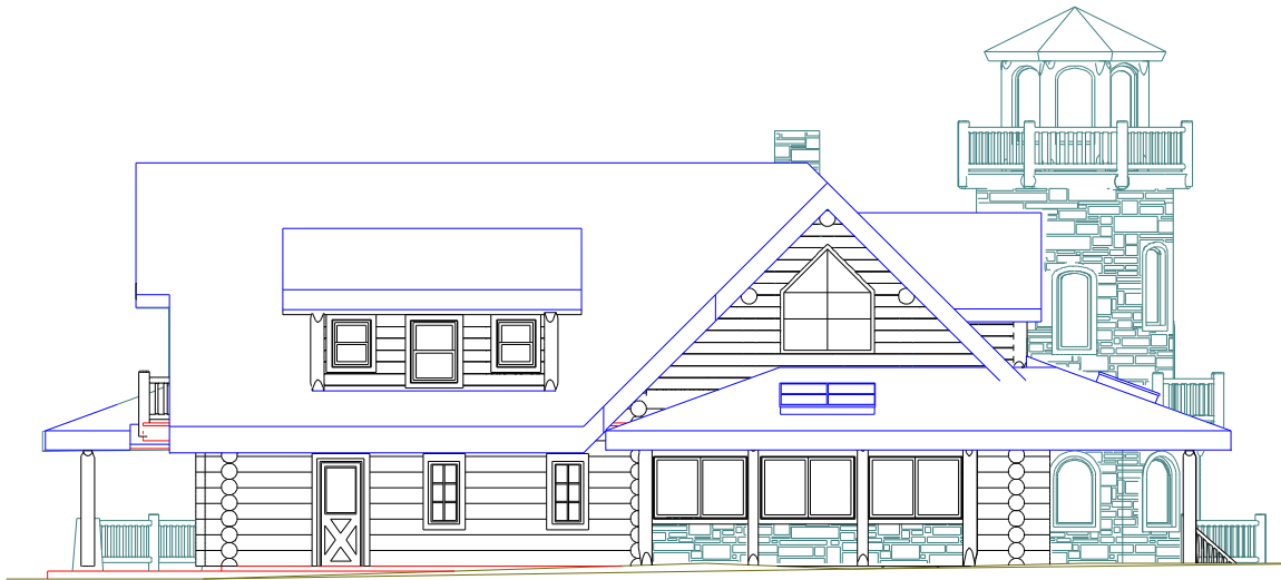
1 NORTH ELEVATION 1/8" = 1'-0"
