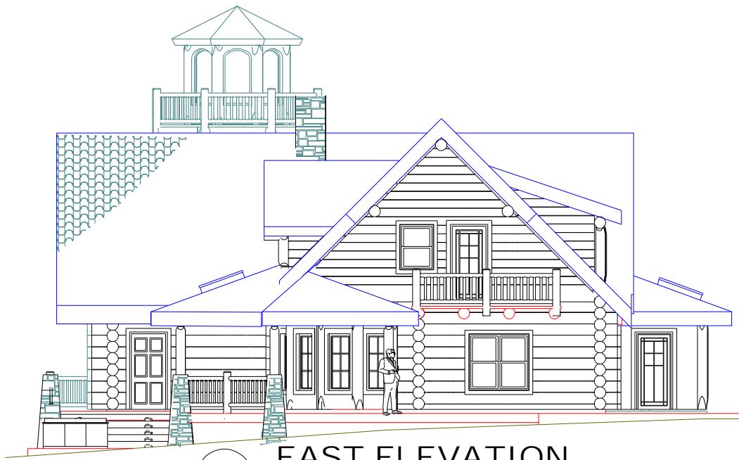
2 EAST ELEVATION 1/8" = 1' - 0"
