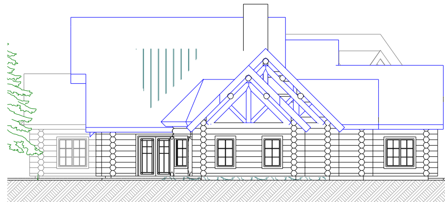
2 WEST ELEVATION 1/8" = 1'-0"
