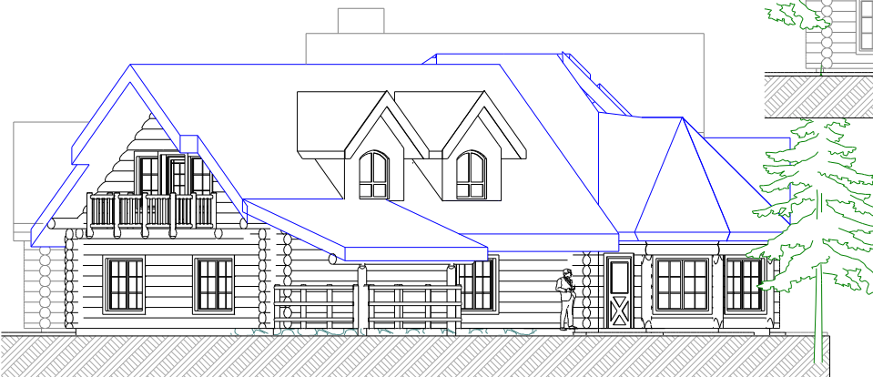
2 EAST ELEVATION 1/8" = 1'-0"
