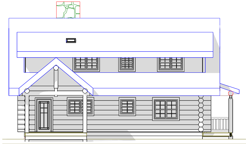
1 NORTH ELEVATION 1/4" = 1'-0"
