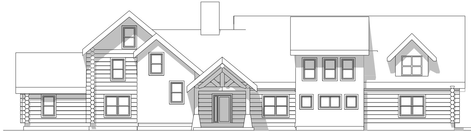
1 SOUTH ELEVATION 1/8" = 1' - 0"
